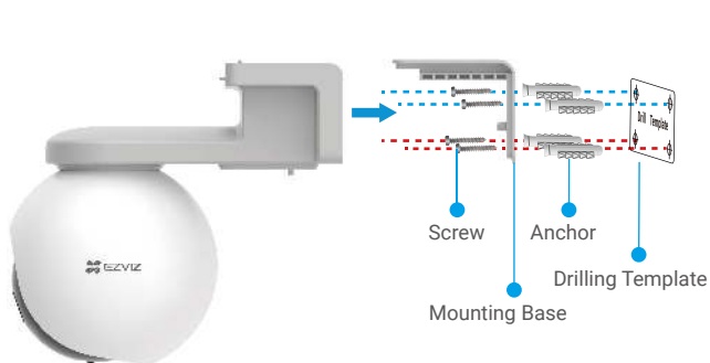
Fig. 2 Wall Mount
