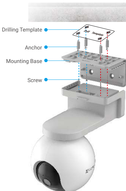
Fig. 1 Ceiling Mount
