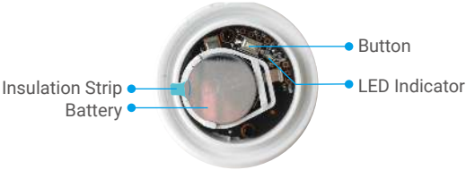
Interior Diagram
