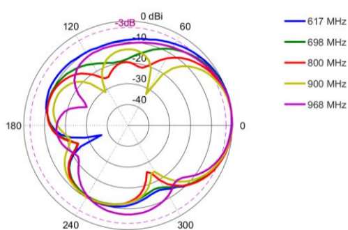
Elevation: 617 – 968 MHz
