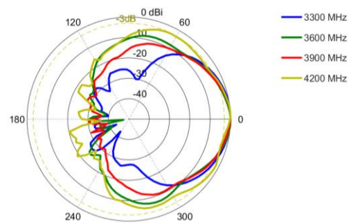
Azimuth: 3300 – 4200 MHz
