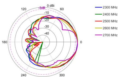
Elevation: 2300 – 2700 MHz
