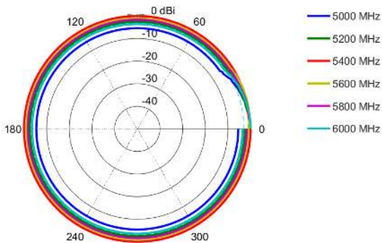
Azimuth: 5000 - 6000 MHz
