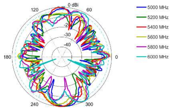
Elevation: 5000 - 6000 MHz
