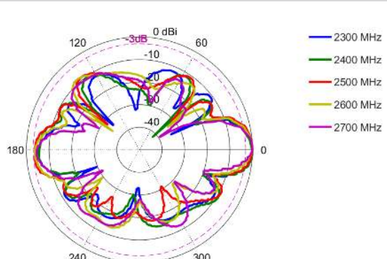
Elevation: 2300 - 2700 MHz
