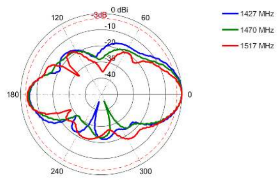
Elevation: 1427 - 1517 MHz
