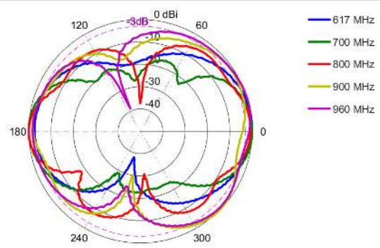
Elevation: 617 - 960 MHz
