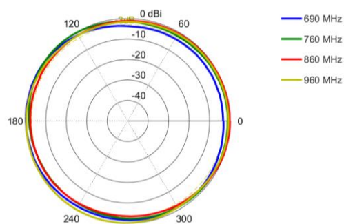
Azimuth: 690 – 960 MHz
