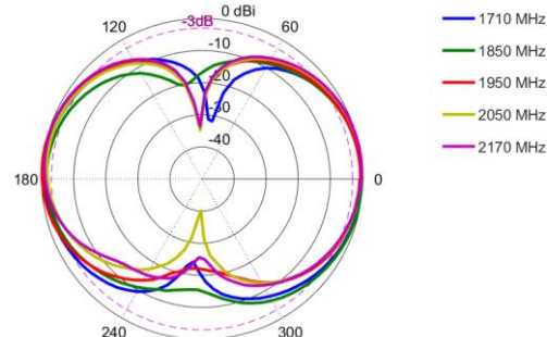
Elevation: 1710 – 2170 MHz
