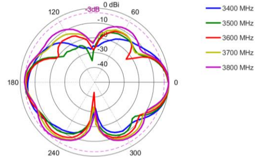
Elevation: 3400 – 3800 MHz
