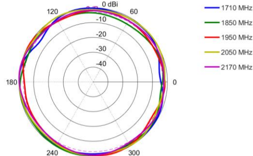
Azimuth: 1710 – 2170 MHz
