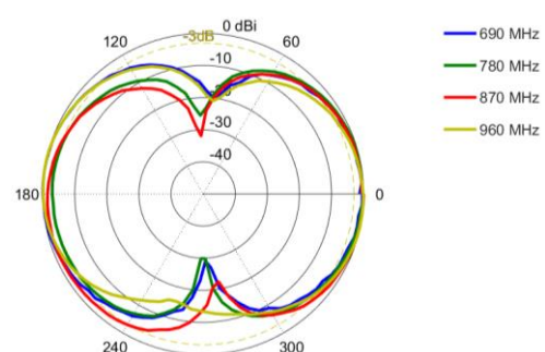
Elevation: 690 – 960 MHz
