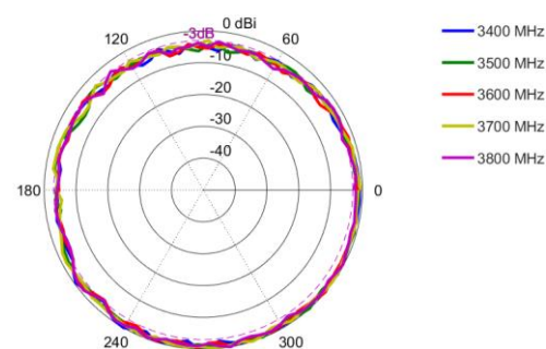
Azimuth: 3400 – 3800 MHz
