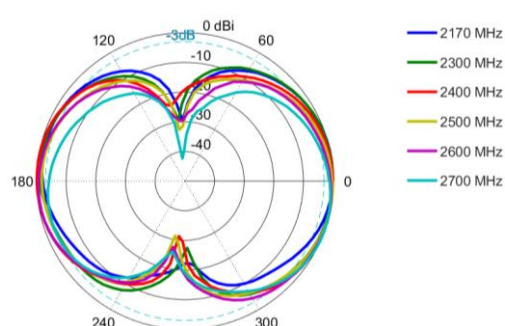
Elevation: 2170 – 2700 MHz
