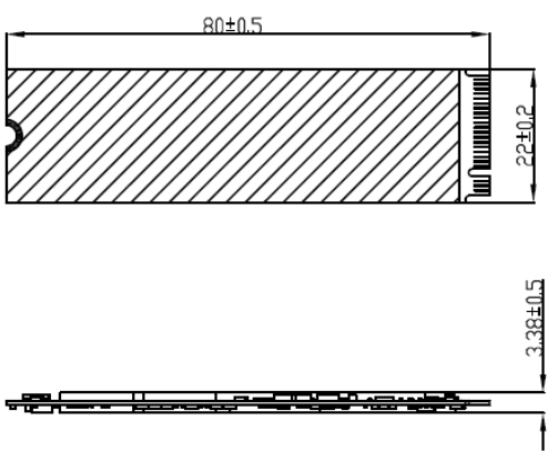
<Without heatsink>
