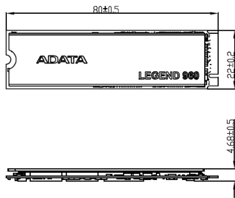
<With heatsink>
