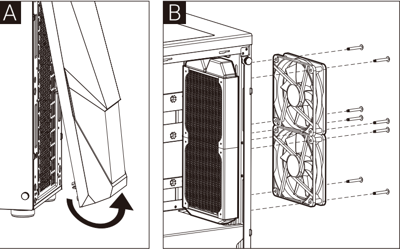
(6a) Install Front Radiator x 1
