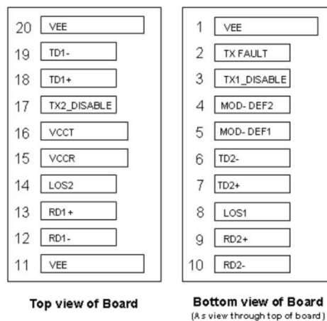
Pinout of Connector Block on Host Board
