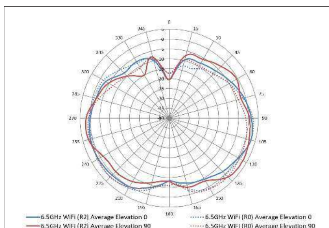
6.5 GHz Wi-Fi antennas patterns (vertical)
