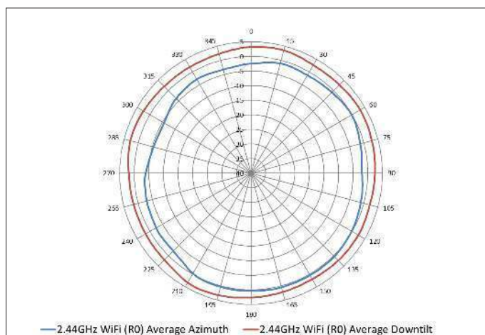
2.44 GHz Wi-Fi antenna patterns (horizontal)
