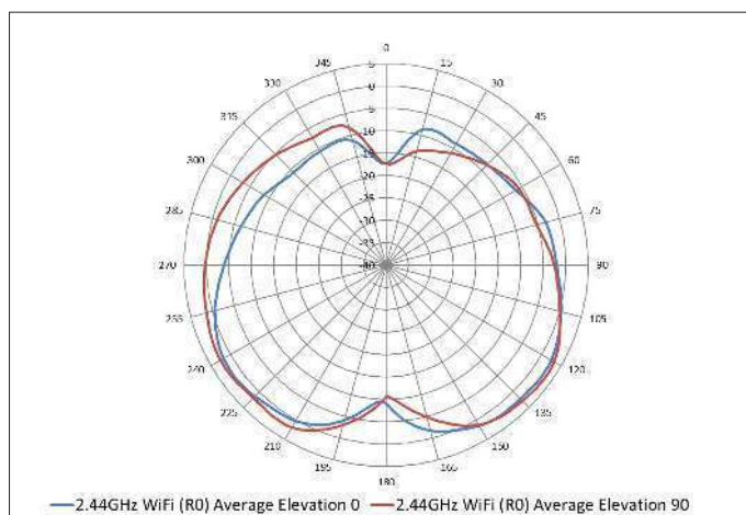
2.44 GHz Wi-Fi antennas patterns (vertical)
